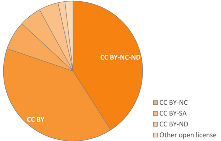
License distribution
