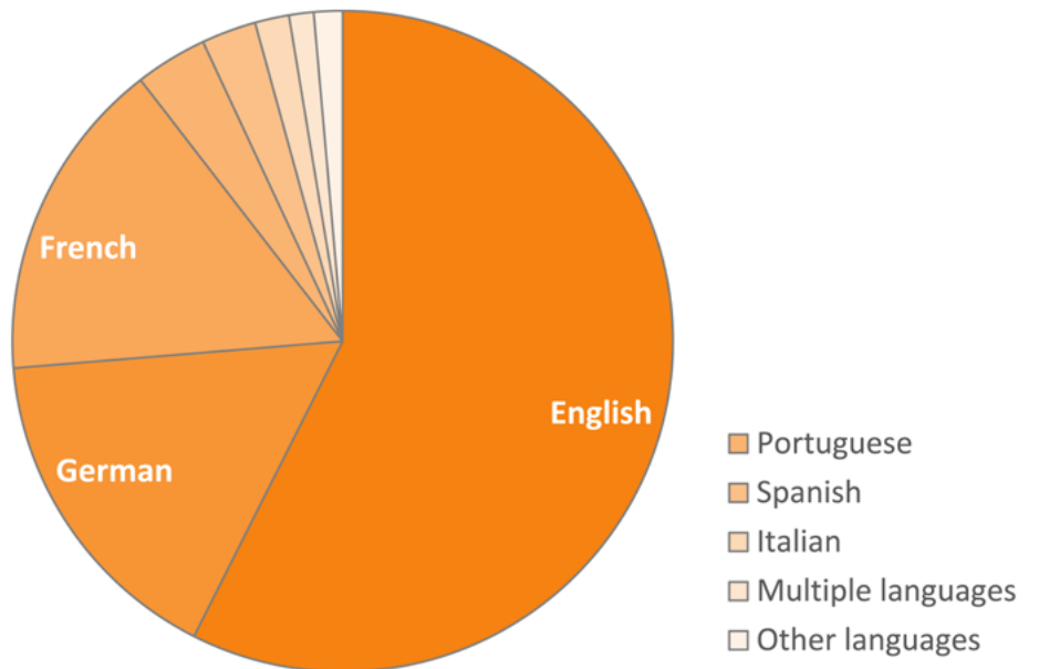
Language distribution
